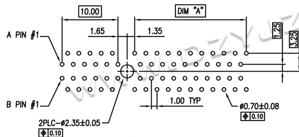
RECOMMENDED PCB LAYOUT SINGLE POST TYPE
