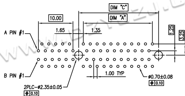
RECOMMENDED PCB LAYOUT DUAL POST TYPE TYPE
